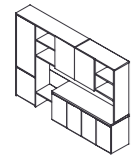
文件柜 DL99(L/R)-2.19 W2560*D500*H1900
