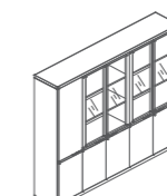
文件柜 EM97-2 W2039*D395*H2000 EM97Z-2 W2039*D395*H2000
