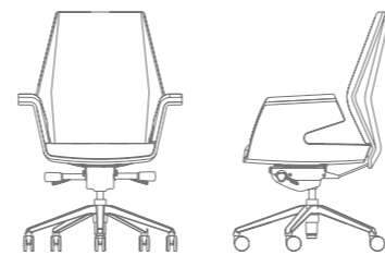
CGL80-1STG (780W*650D*H980)
