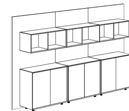
EI98 文件柜 Filing Cabinet 3400(W)*490(D)*2000(H)
