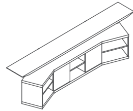
Filing Cabinet 矮柜 W3250*D680*H890 (mm)
