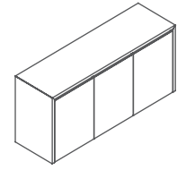
Filing Cabinet 矮柜 W1600*D480*H740 (mm)
